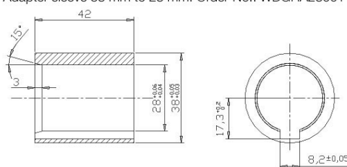
Adapter sleeve 38 mm to 28 mm: Order-No.: WDGHA28001
