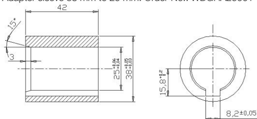
Adapter sleeve 38 mm to 25 mm: Order-No.: WDGHA25001
