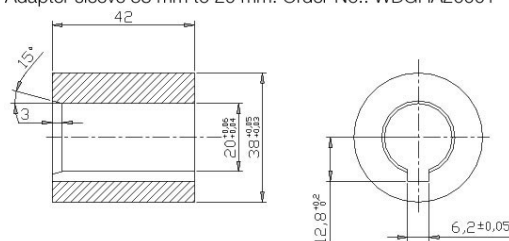
Adapter sleeve 38 mm to 20 mm: Order-No.: WDGHA20001
