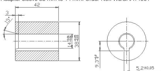
Adapter sleeve 38 mm to 14 mm: Order-No.: WDGHA14001
