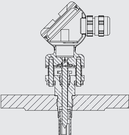
Flange version without cooling element
