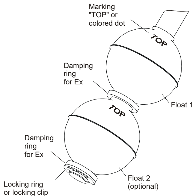
Figure 8: Locking clip, damping ring
