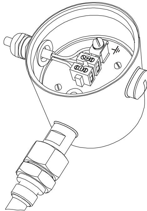
Figure 11: Terminal box.
