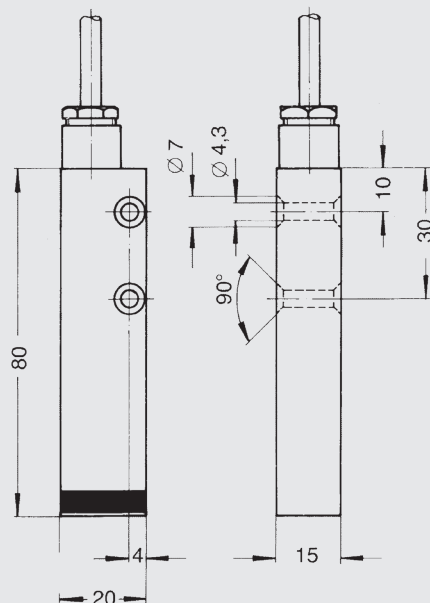
Models MSA-FLS-AL and MSA-FLU-AL
