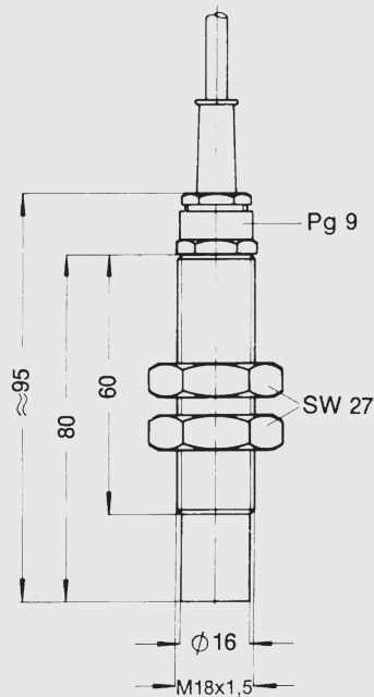
Models MSA-GMS 18 and MSA-GMU 18
