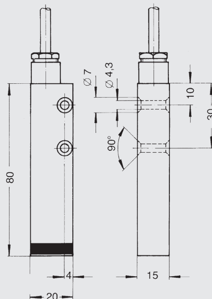
Models MSA-FLSM-AL and MSA-FLUM-AL
