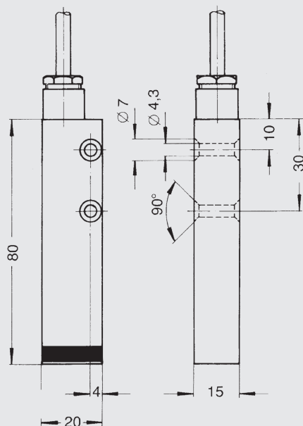
Models MSA-DRS and MSA-DRU
