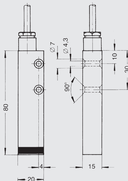
Models MSA-DRSM and MSA-DRUM
