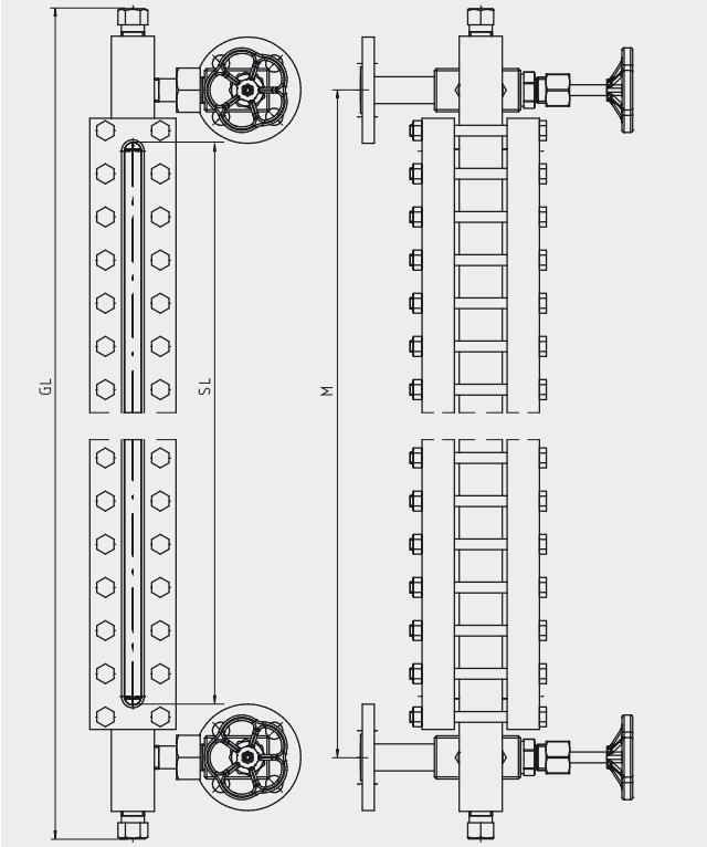
Version with valve head, lateral, model LGV-52
